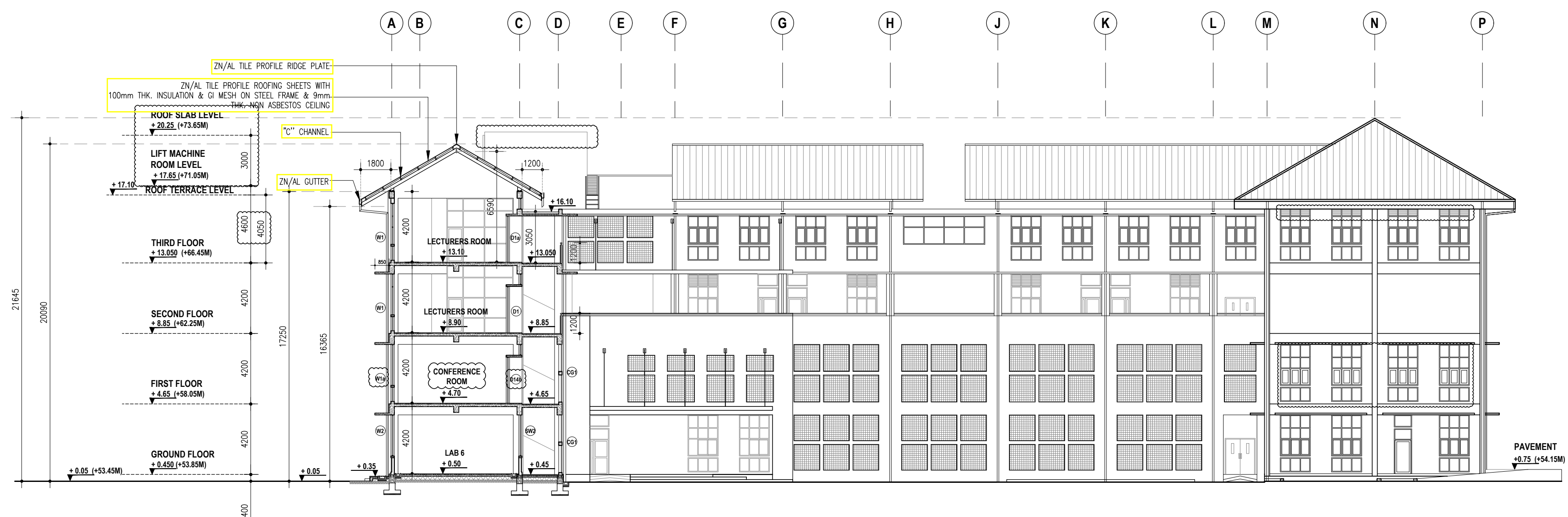
SECTION B-B
