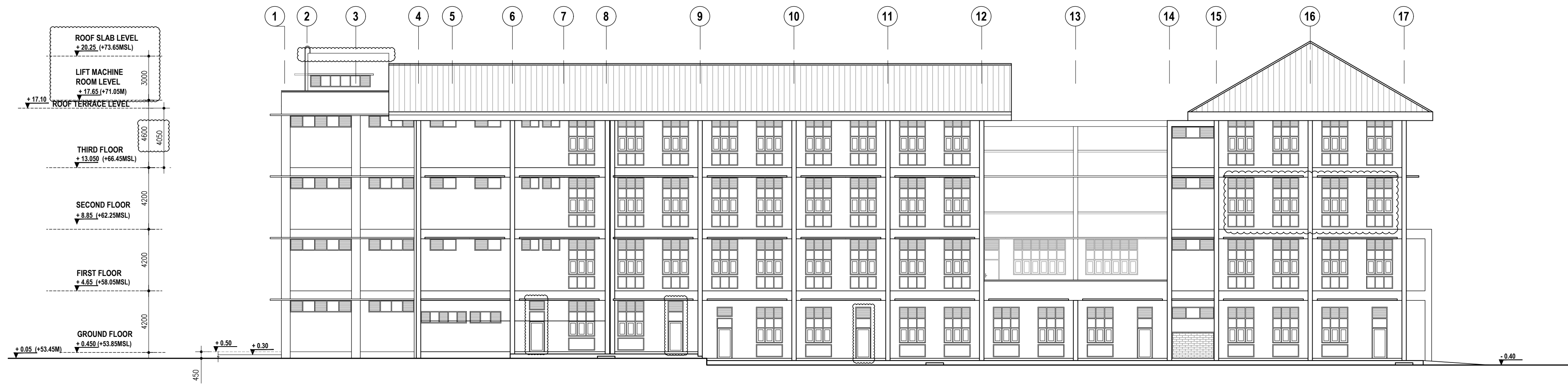
ELEVATION C
